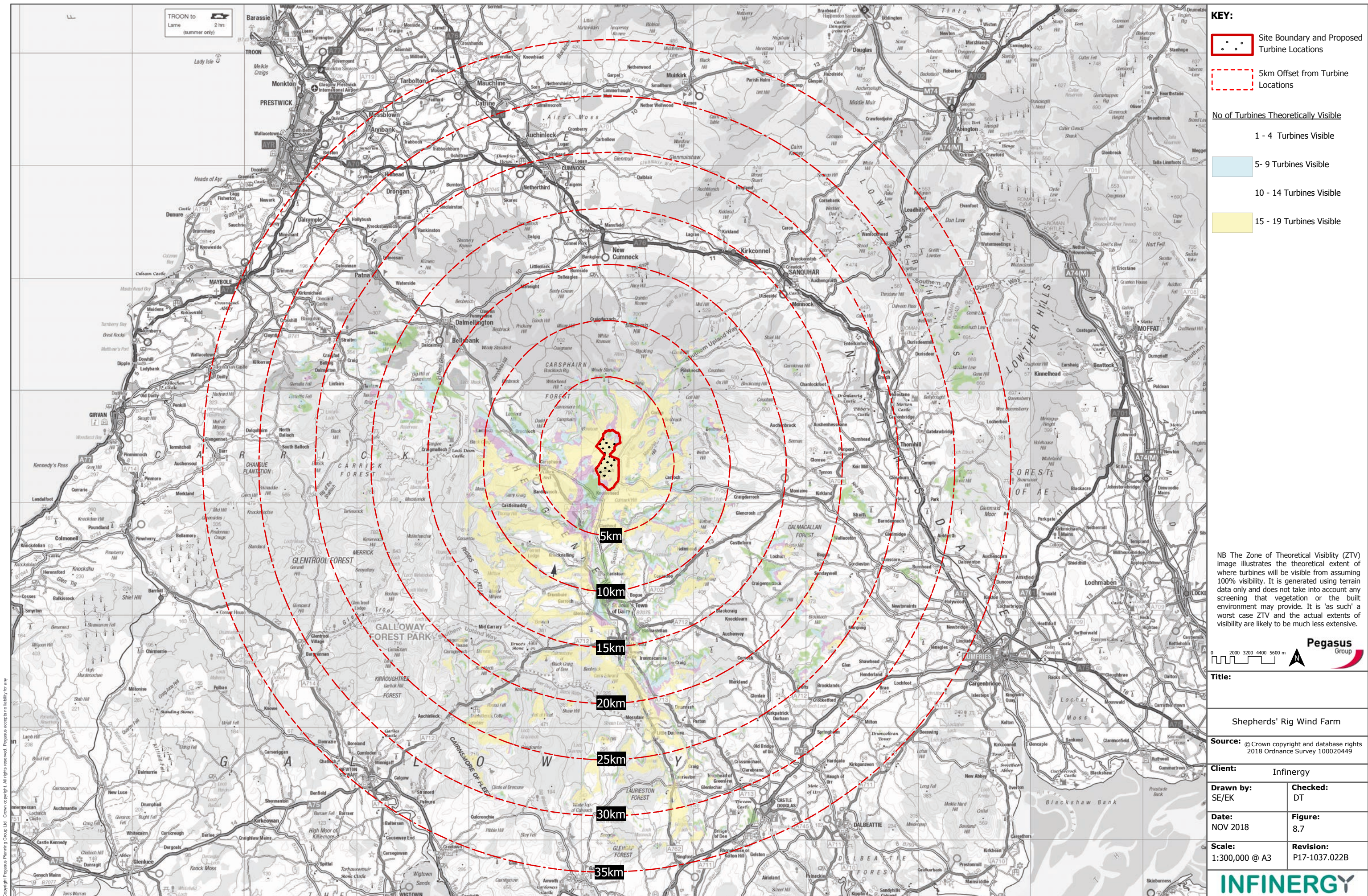
Figure 8.7 Blade Tip ZTV to 35 km
